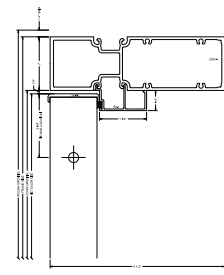
2650 HEAD
