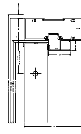
1450 HEAD
