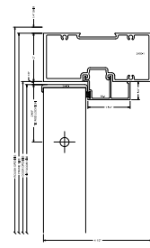
2450 HEAD
